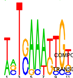
upstream meme PSSM #2; e=70
