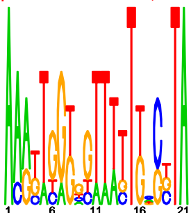
upstream meme PSSM #1; e=0.49
